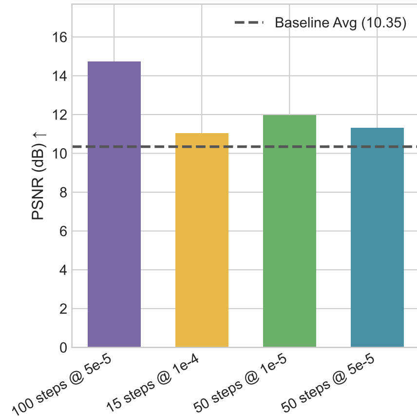
PSNR Comparison
