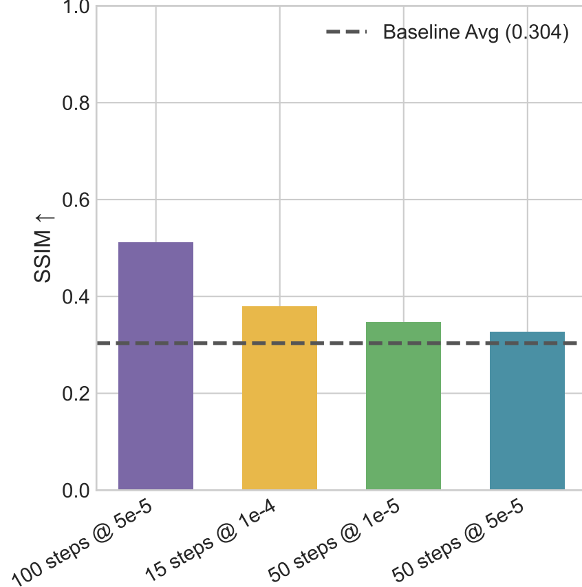
SSIM Comparison
