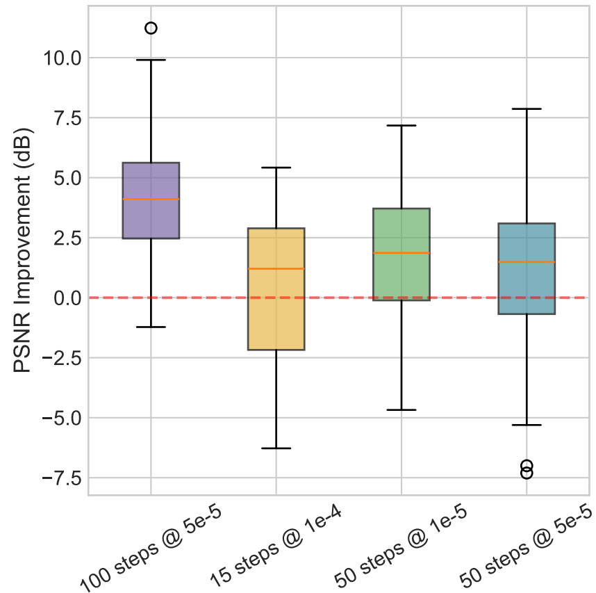
PSNR Improvement Distribution
