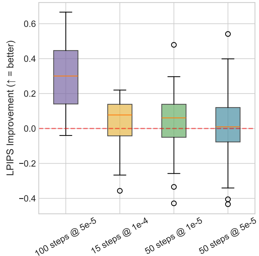
LPIPS Improvement Distribution
