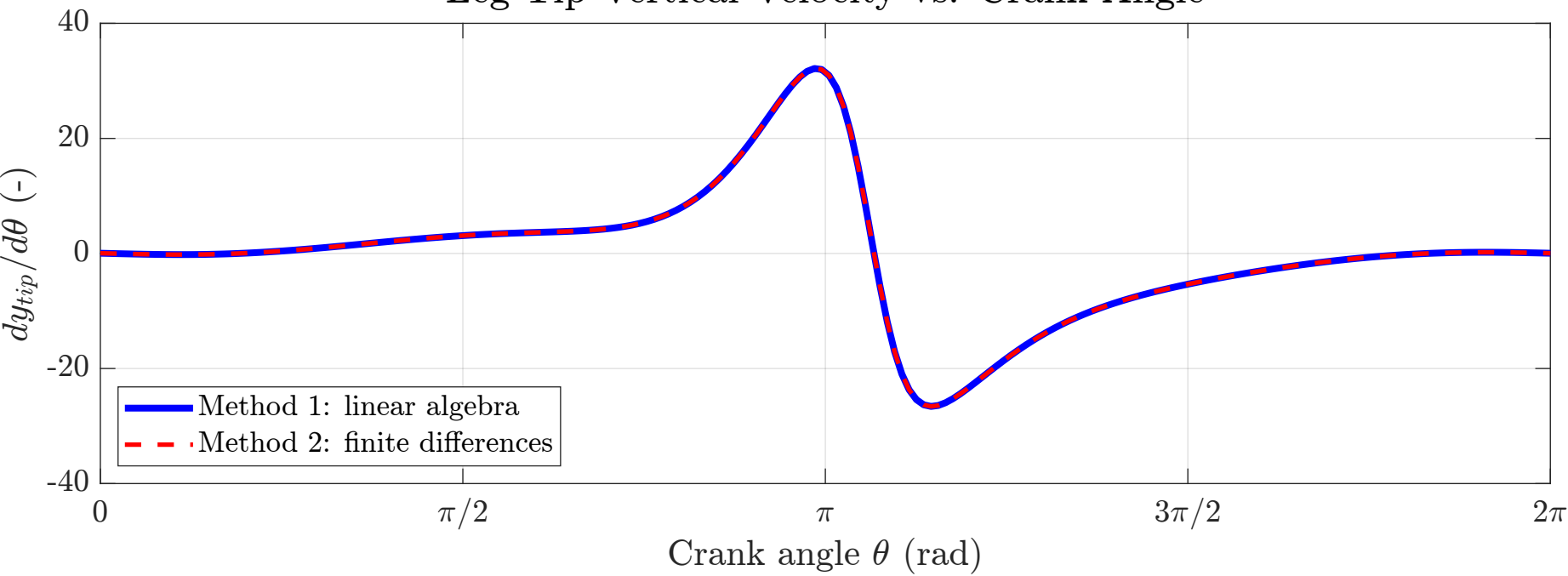
Leg Tip Vertical Velocity vs. Crank Angle
