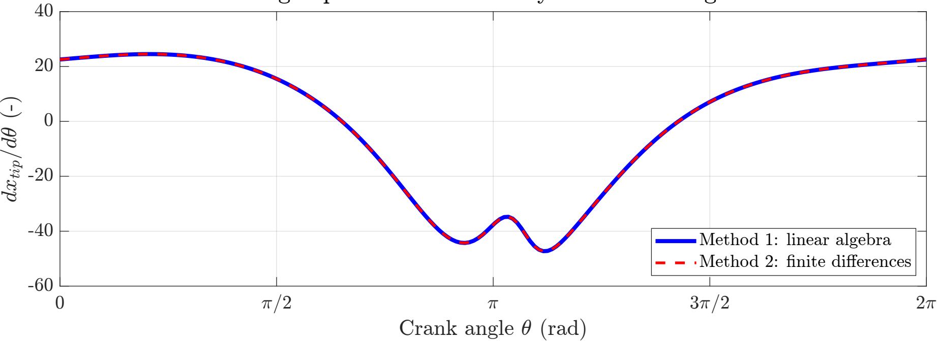
Leg Tip Horizontal Velocity vs. Crank Angle
