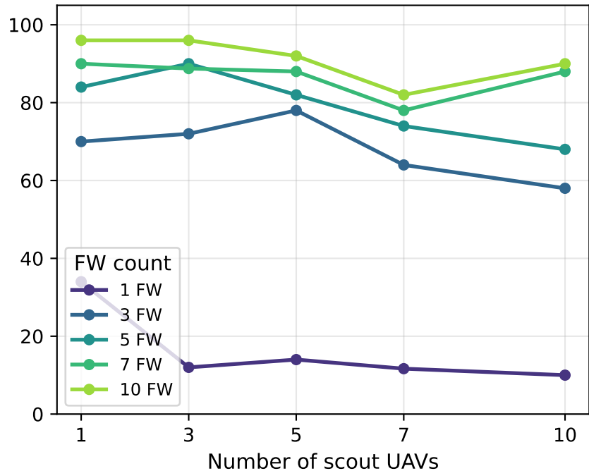
(a) Effect of scout count on suppression
