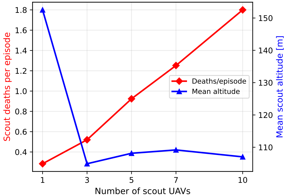
(b) Scout survival & altitude
