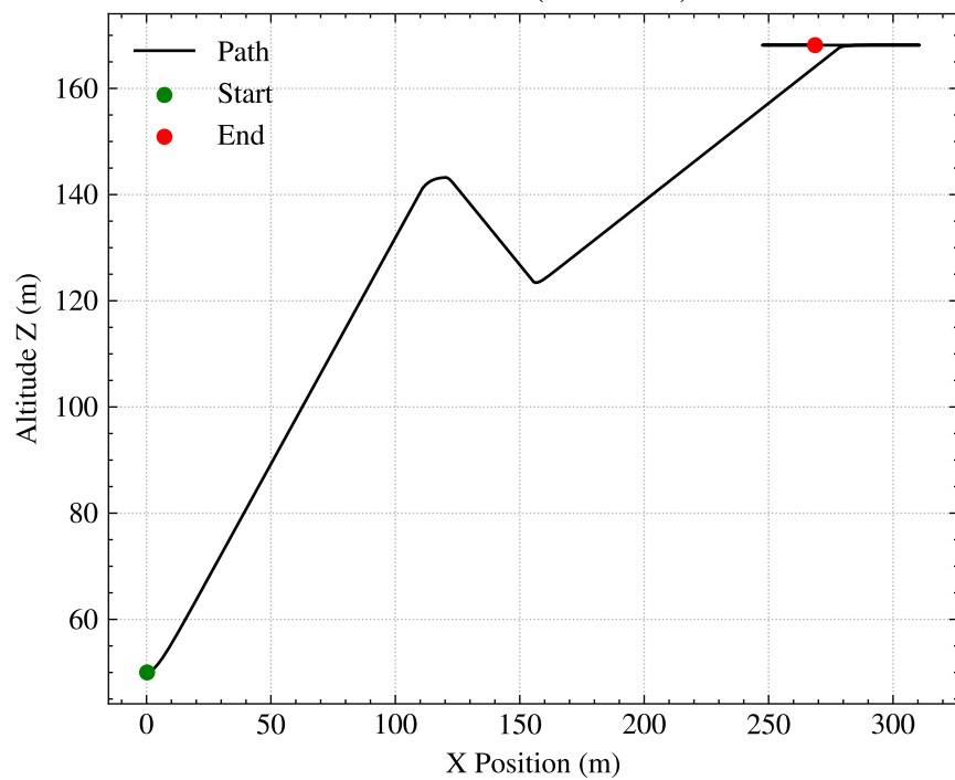
Side View (Elevation)
