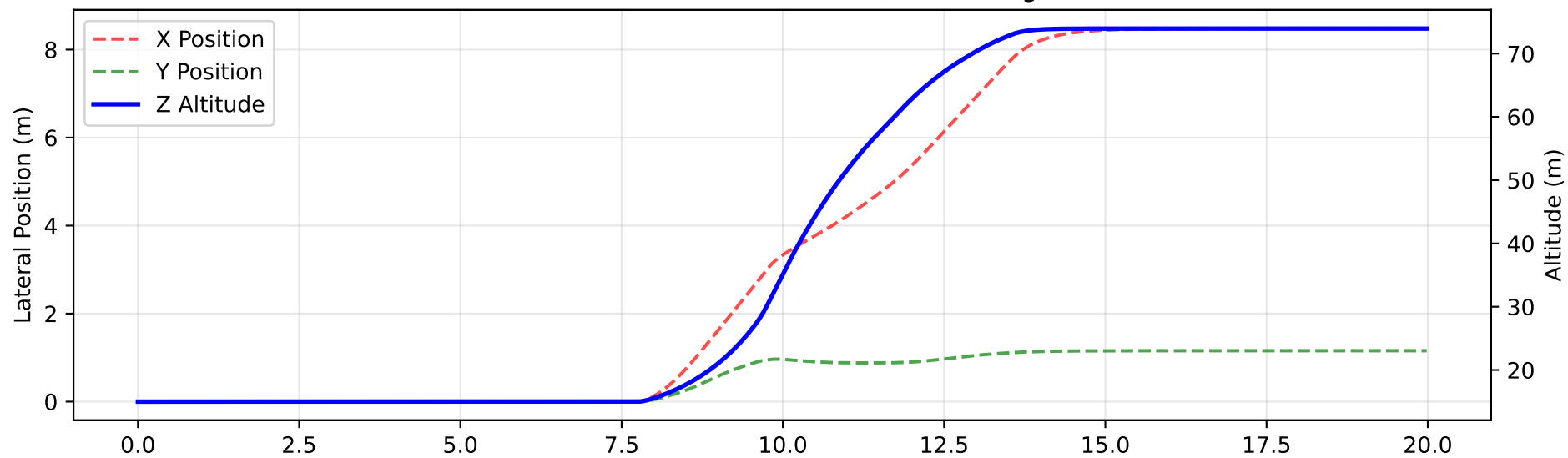
Quad Low (15m above fire) - Hovering
