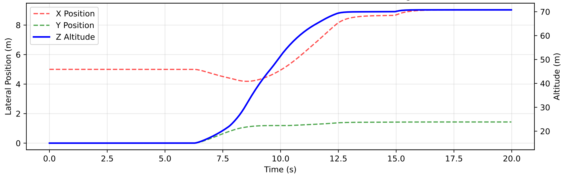
Quad High (35m above fire) - Hovering
