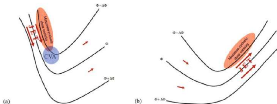
Figure 2.13. Idealized schematics of (a) a digging trough and (b) a lifting trough. Geopotential (solid contours), select wind vectors (arrows), and the locations of vorticity and vorticity advection maxima are labeled (from Bluestein 1993).
