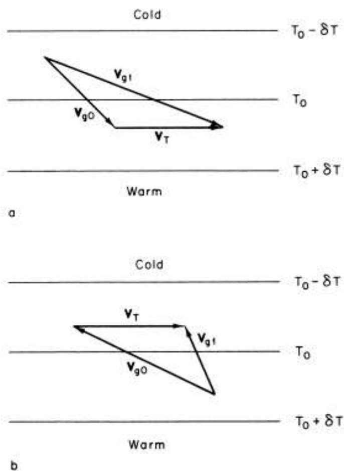
Slika 15.8: a) backing in b) veering.
