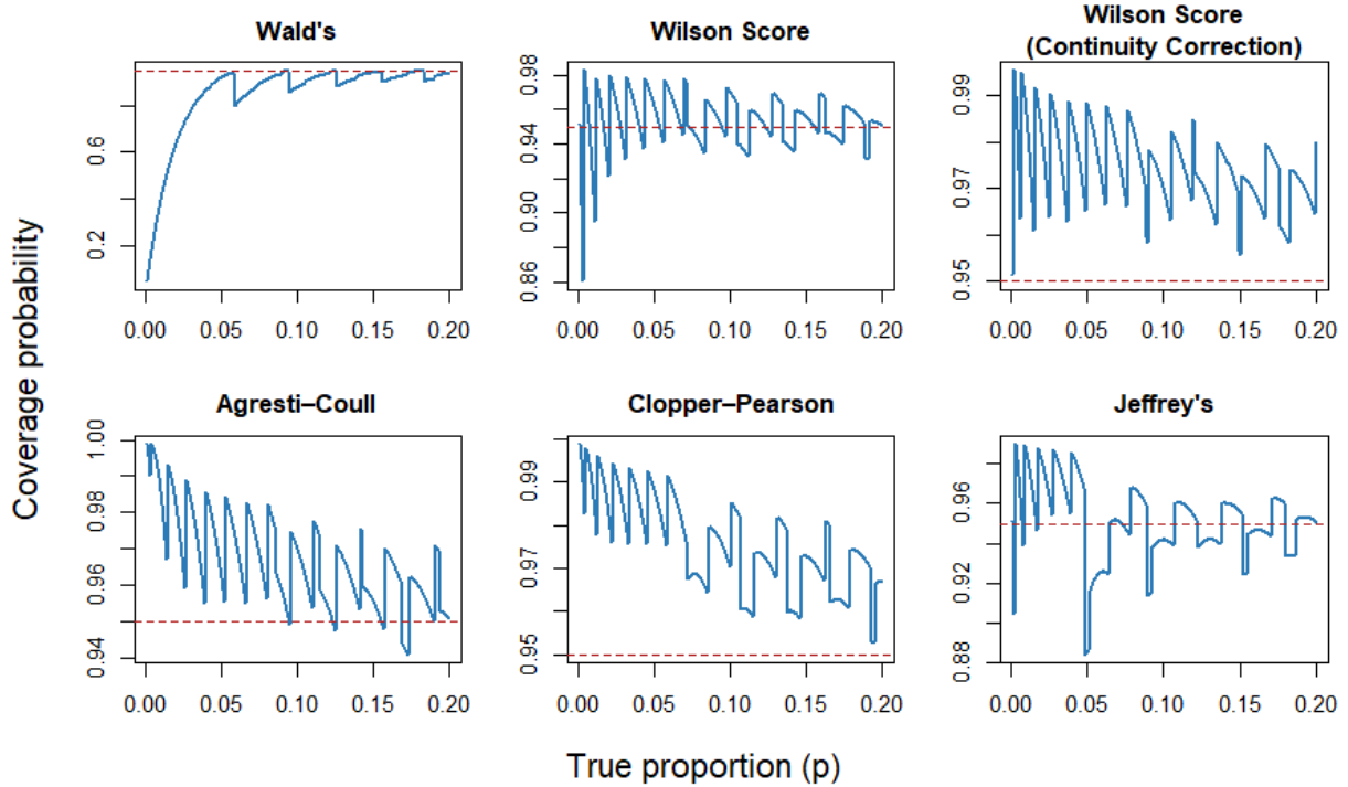
Figure 4: Coverage probability curves for six binomial confidence interval methods at n = 50 , evaluated across true proportions p in 0.001, \dots, 0.200 . The dashed red line indicates the nominal 95% level.
