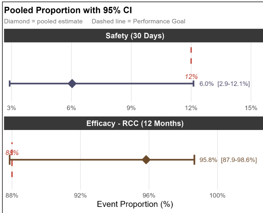
Figure 3: Pooled event proportions with 95% confidence intervals for the safety and efficacy endpoints.
