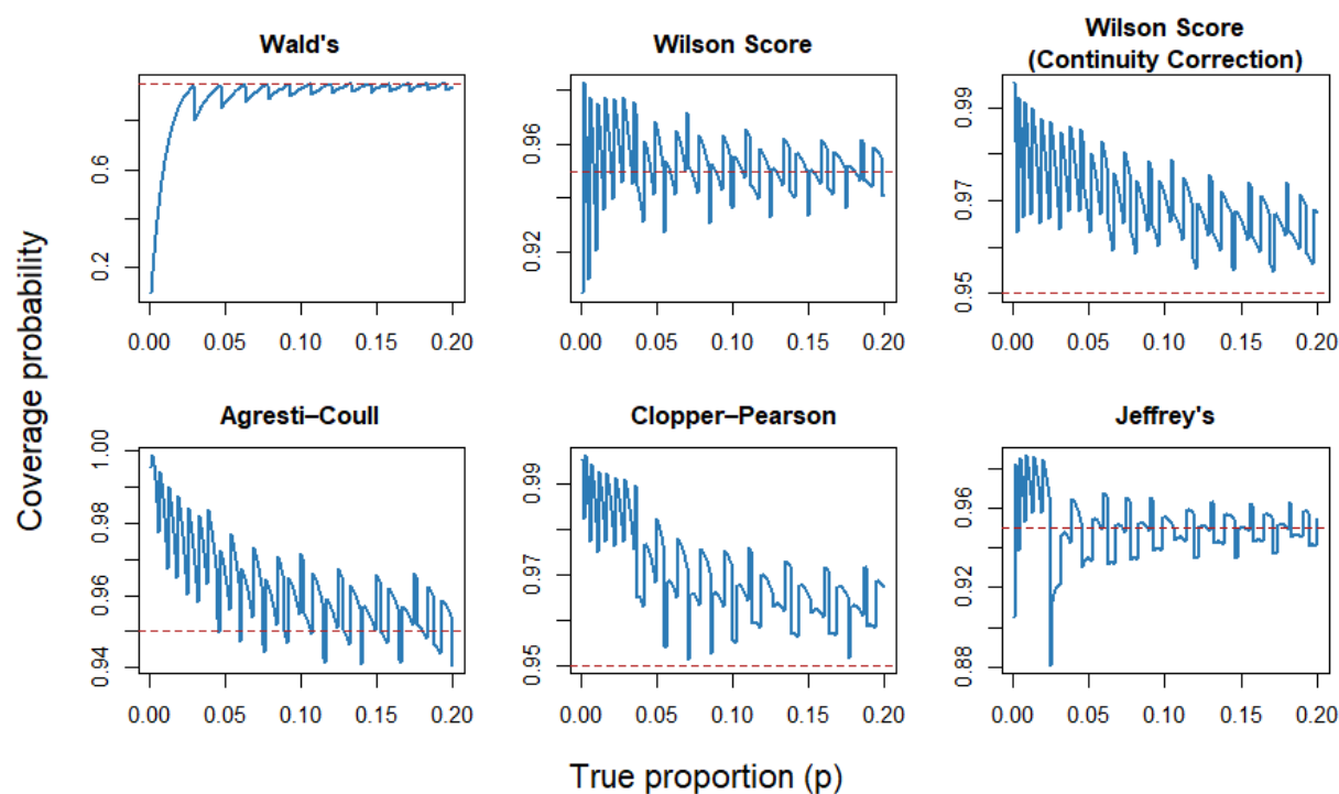
Figure 5: Coverage probability curves for six binomial confidence interval methods at n = 100 , evaluated across true proportions p in 0.001, ..., 0.200. The dashed red line indicates the nominal 95% level.
