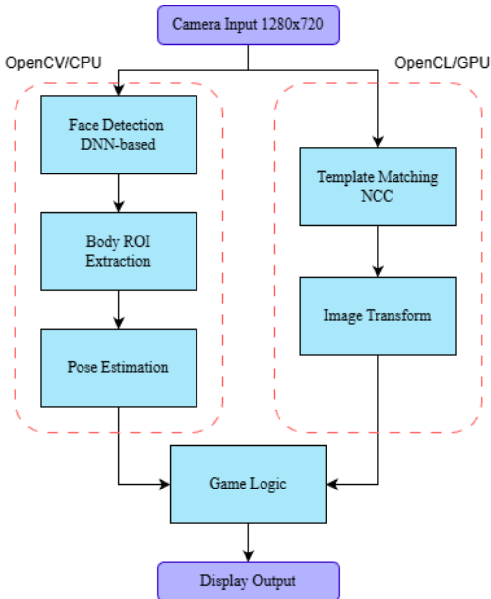
Figure 1: System architecture and data flow diagram
