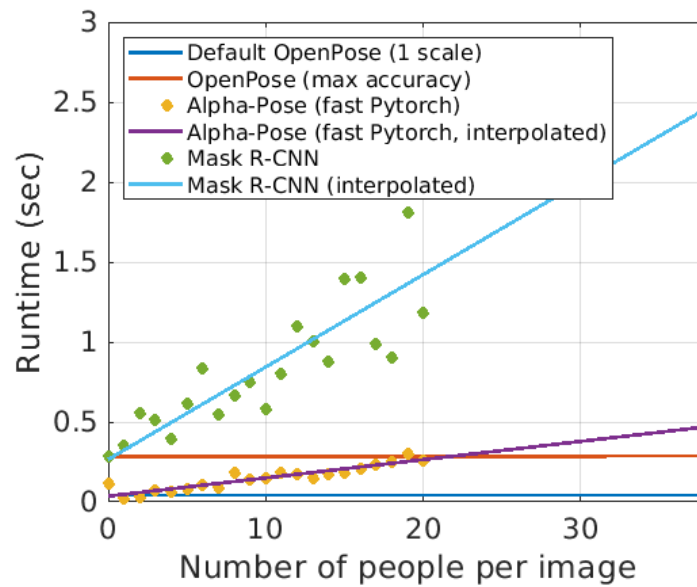
Figure 2: openpose run time
