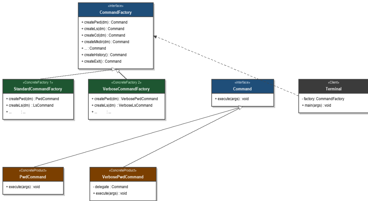
Diagrama de Classes — Abstract Factory: Terminal-linux
