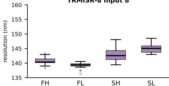
TRMISR-8 input 8
