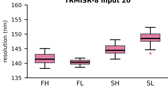
TRMISR-8 input 20
