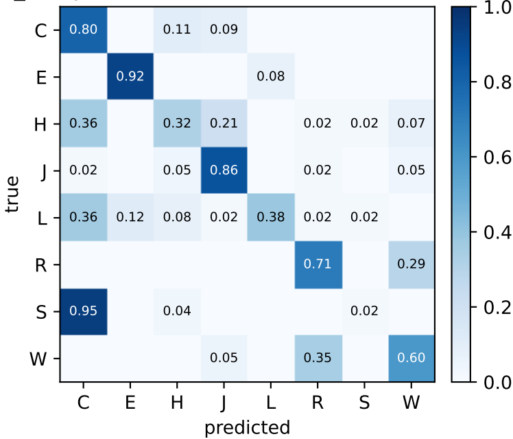
C1_sharplike — test confusion (row-normalized)
