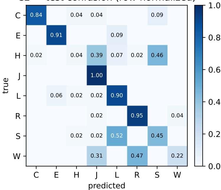
C2 — test confusion (row-normalized)
