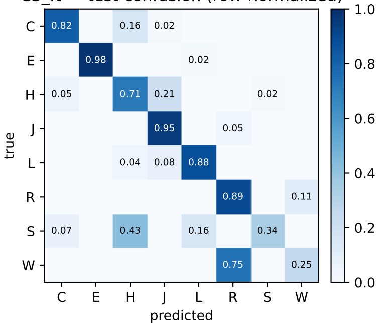
C3_ft — test confusion (row-normalized)
