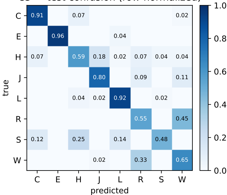
C3 — test confusion (row-normalized)
