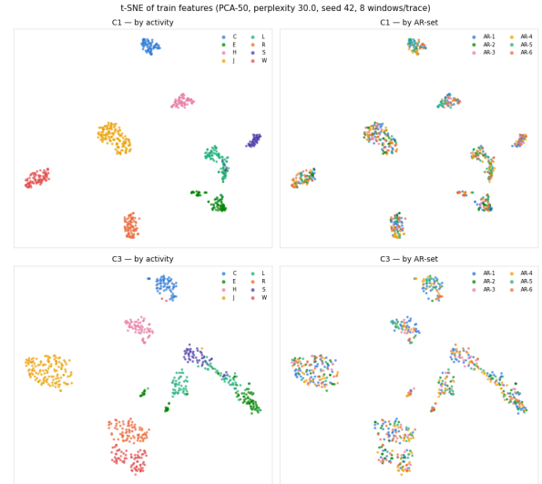
Fig. 3: t-SNE [10] of train features, identical recipe; top row C1 (CE), bottom row C3 (SupCon). Left, by activity : both form tight clusters, but C3’s L/S/E clusters chain into one filament instead of three separable blobs — the geometric counterpart of its lower linear-probe score. Right, the same points by capture set : colours are uniformly mixed inside every cluster, in both encoders — no domain sub-structure exists for an adversary to remove.
