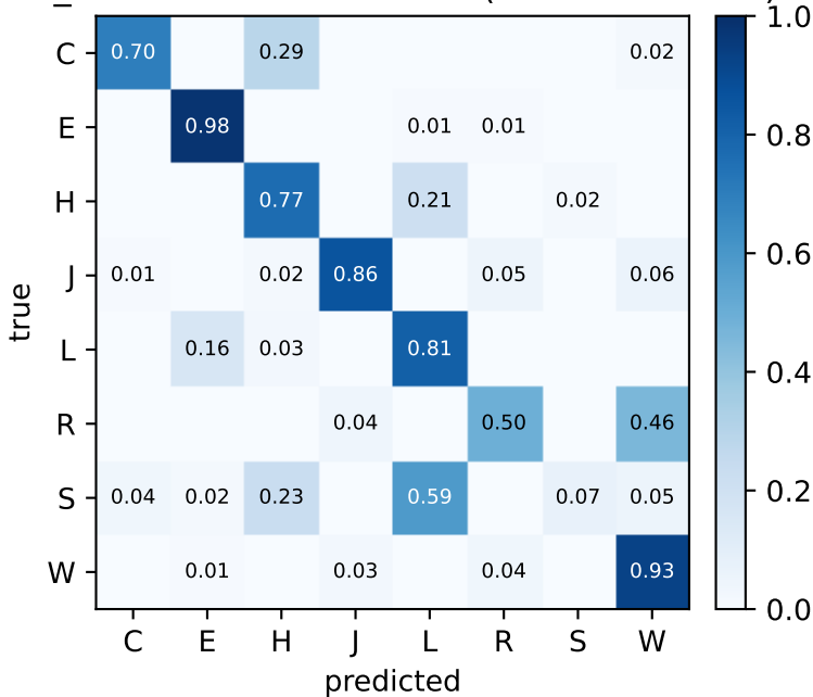
C1_s6out — test confusion (row-normalized)
