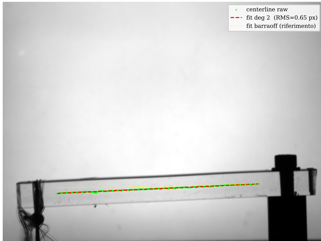
barraon centerline + fit (unified)
