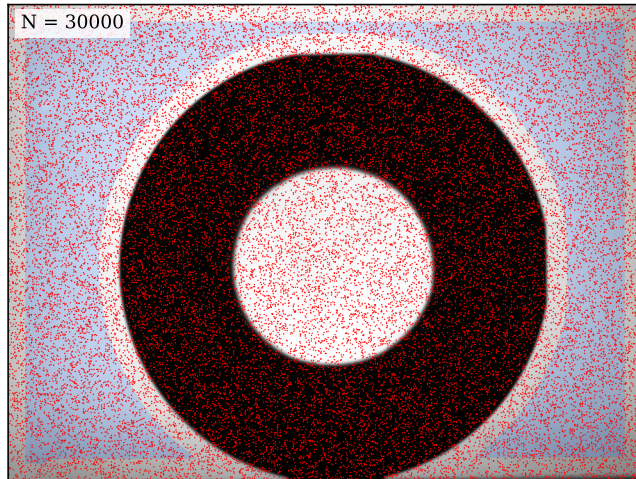
lambdaquarti_50deg / G — N=30000
