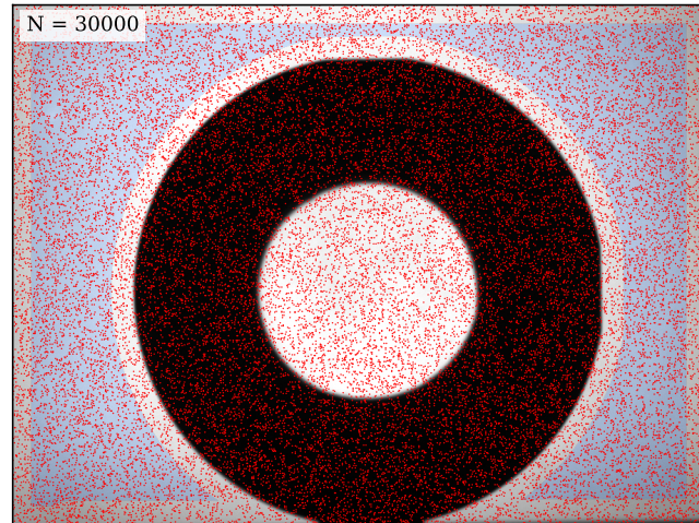
lambdaquarti_50deg / B — N=30000
