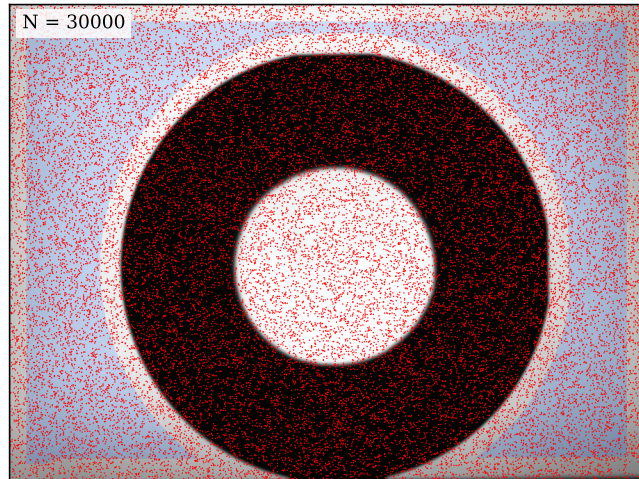
lambdaquarti_50deg / R — N=30000
