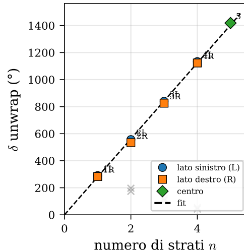
Fit \delta = m n (+7 unwrap) m = 280.80^\circ/\text{strato} , R^2 = 0.999
