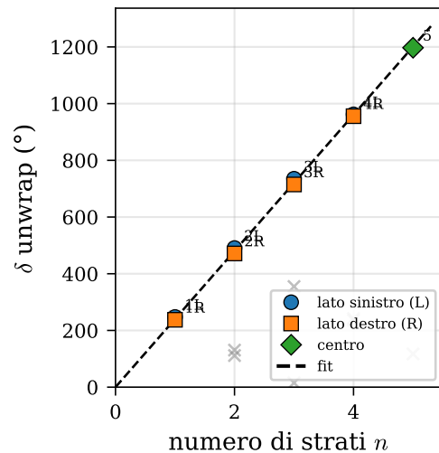
Fit \delta = m n (+7 unwrap) m = 240.20^\circ/\text{strato} , R^2 = 0.999
