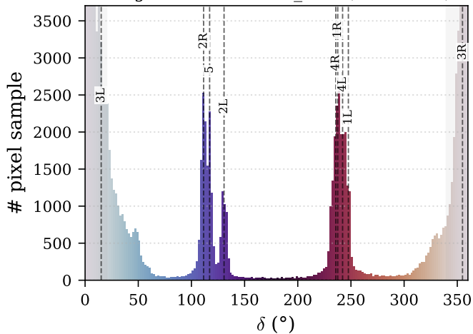
Istogramma \delta — strati_v2/R ( \lambda=626 nm)
