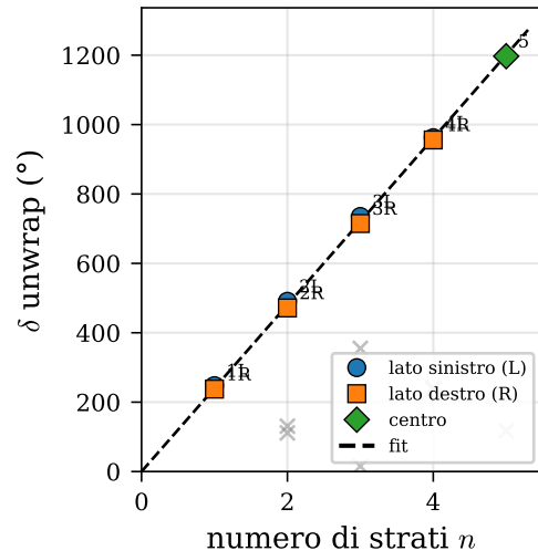
Fit \delta = m n (+7 unwrap) m = 240.20^\circ/\text{strato} , R^2 = 0.999
