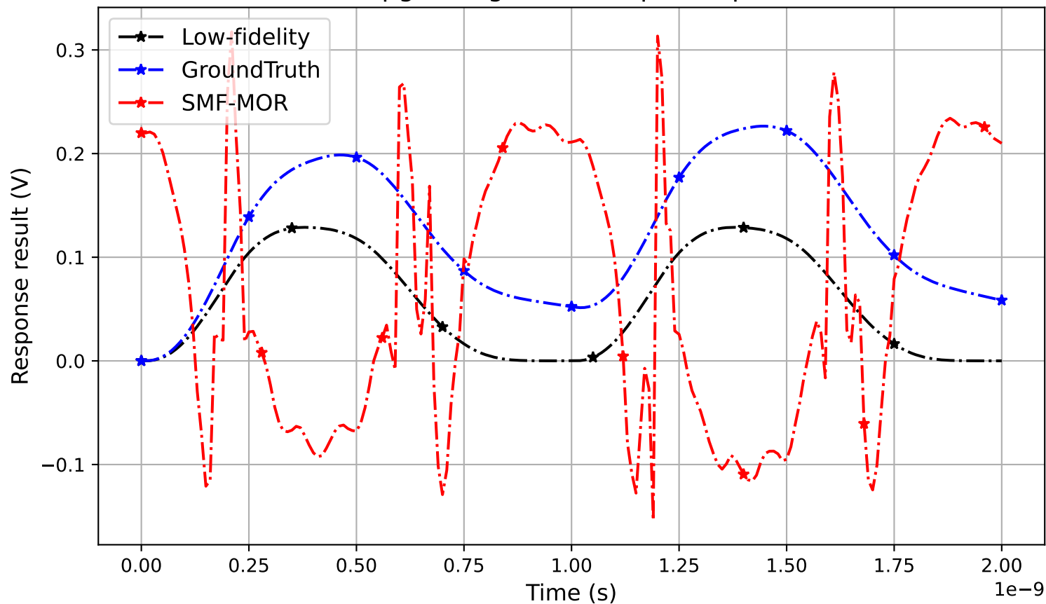
ibmpg3t single-Port output response
