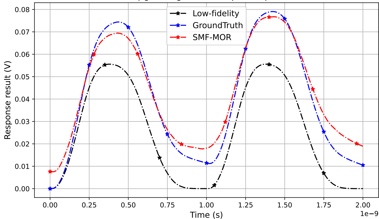
ibmpg6t single-Port output response
