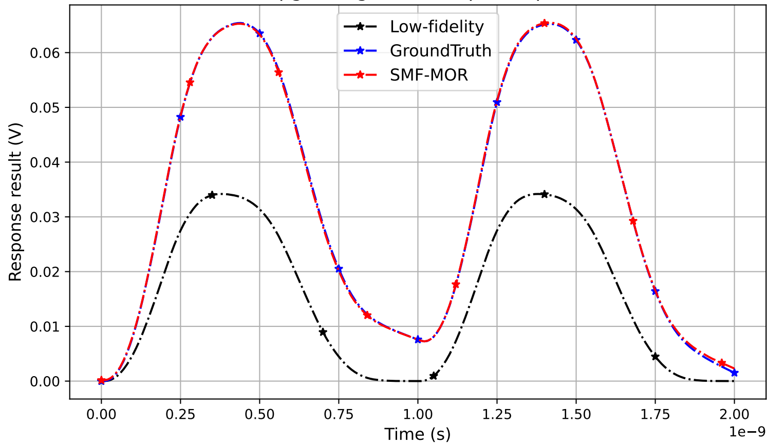
ibmpg5t single-Port output response
