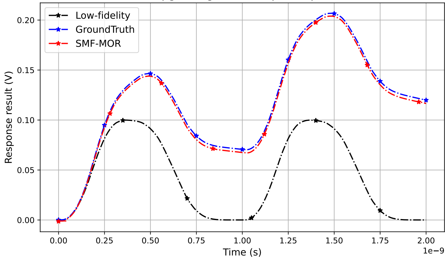
ibmpg2t single-Port output response
