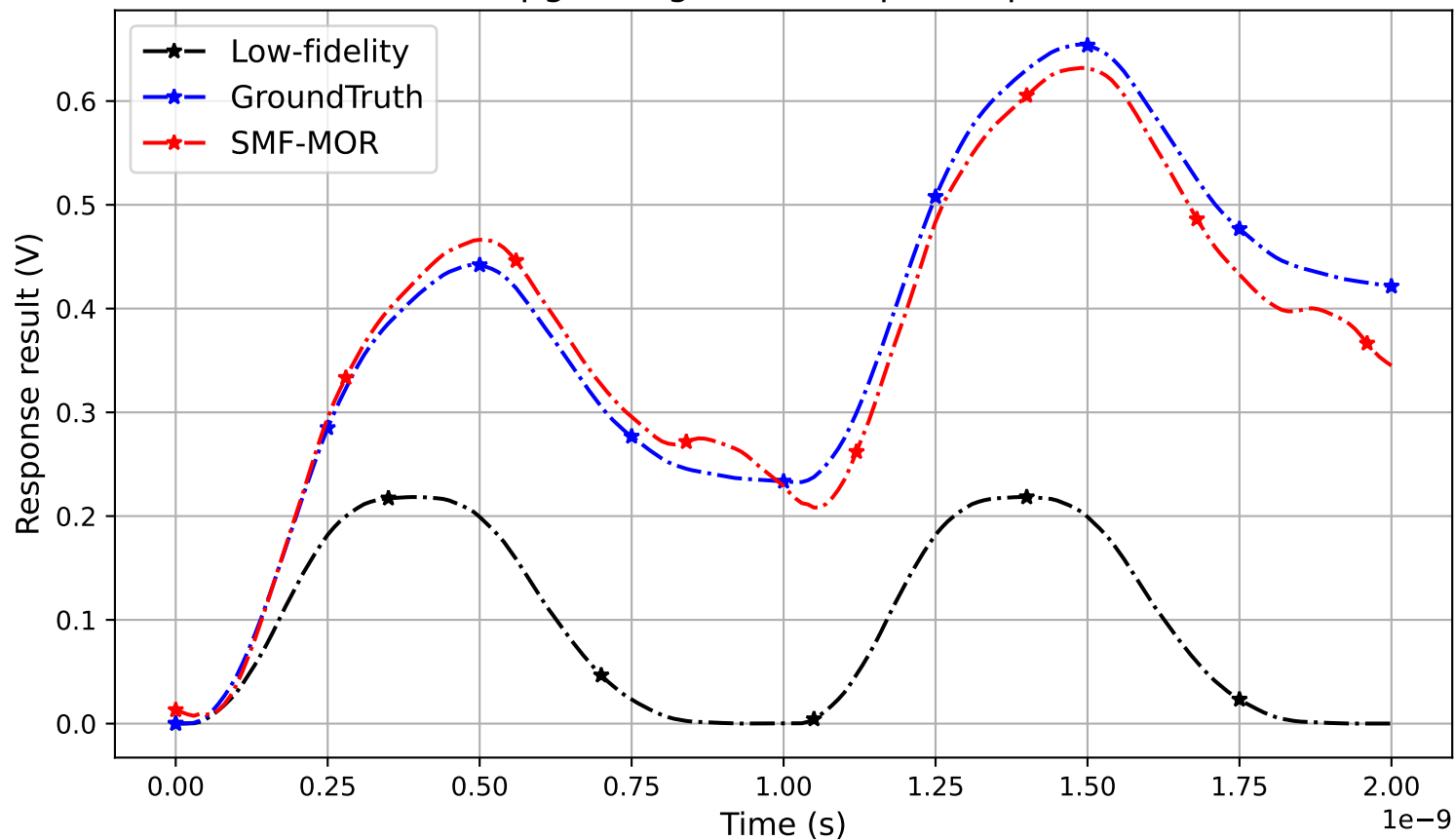
ibmpg1t single-Port output response
