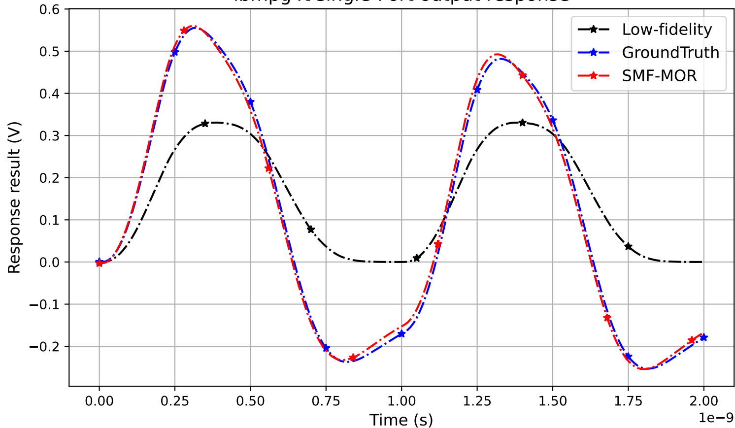
ibmpg4t single-Port output response
