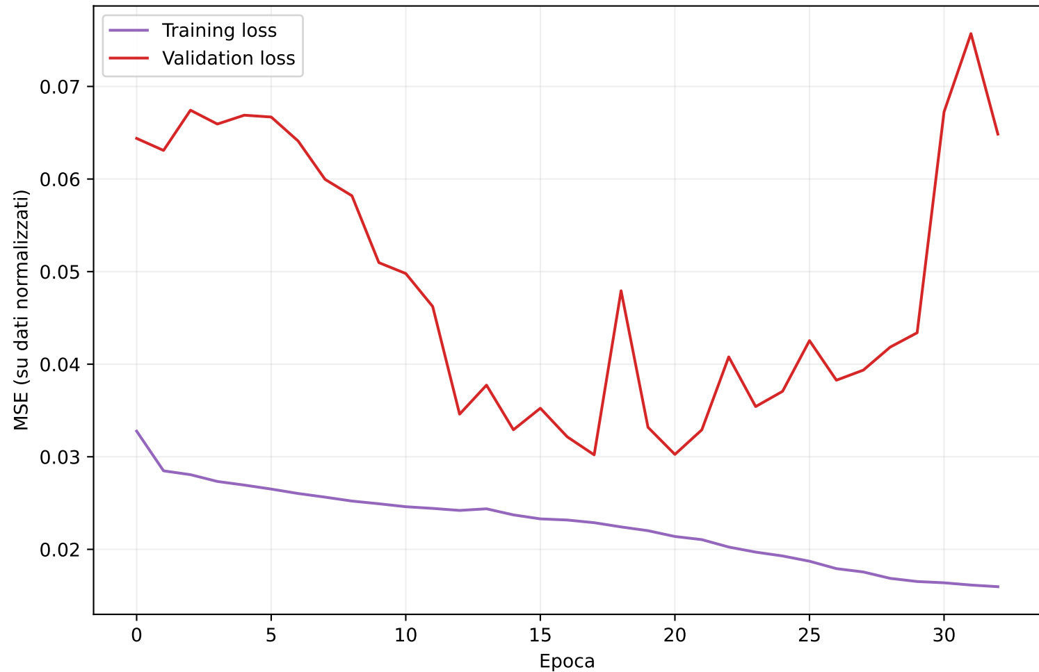
Fig. 3 — Training loss curve, BiLSTM-CNN-Attention, H=1
