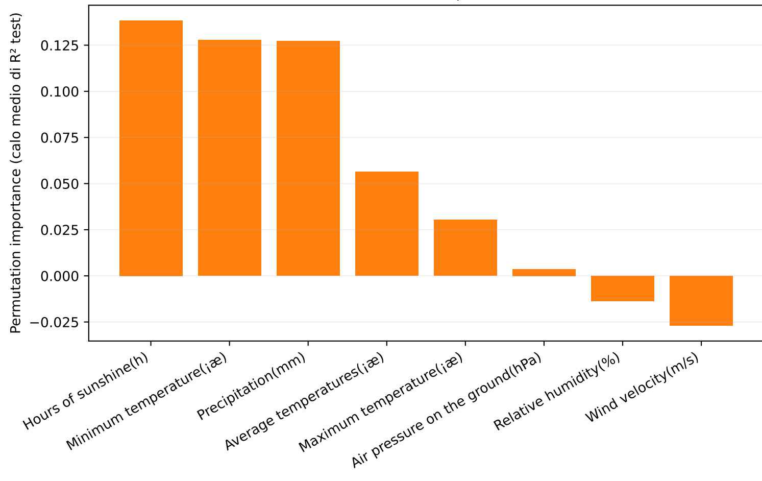
Fig. 4 — Feature importance, Gradient Boosting, H=1 (somma sui 20 timestep della finestra)
