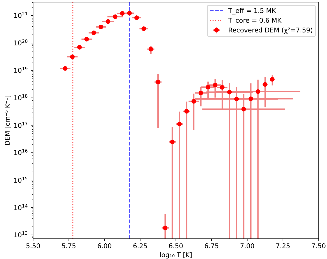
Recovered DEM from \kappa=2.5 synthetic observations
