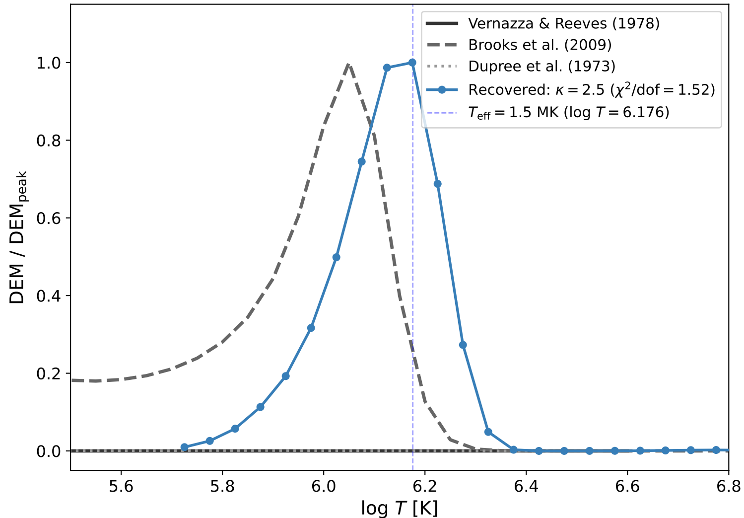
Recovered DEM from \kappa = 2.5 plasma vs published quiet Sun
