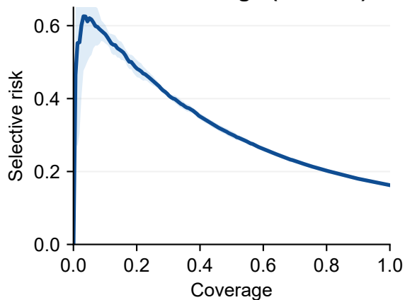
C Acceptance reliability
