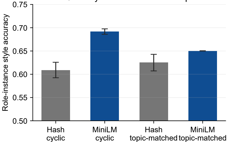
PersonaChat style attribution under topic control
