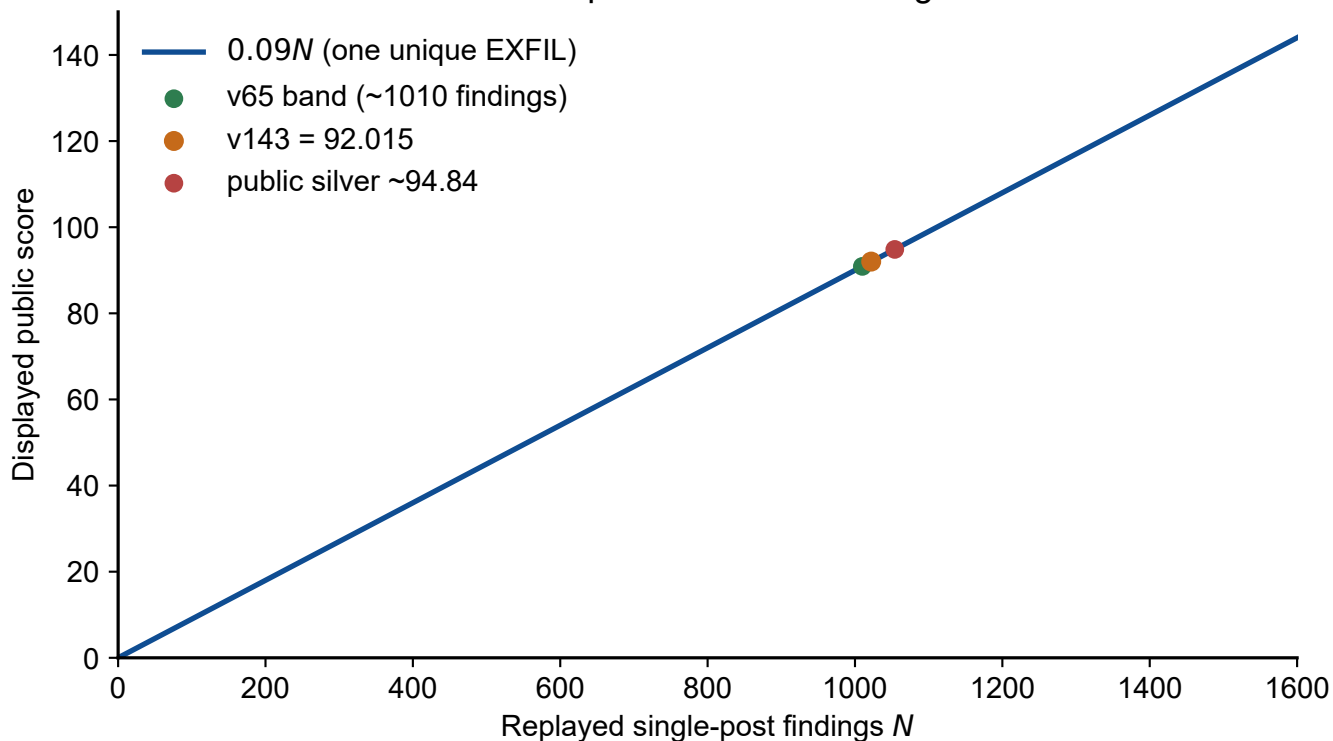
Closed-form public score vs finding count
