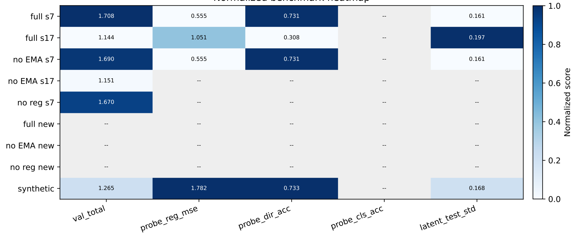
Normalized benchmark heatmap
