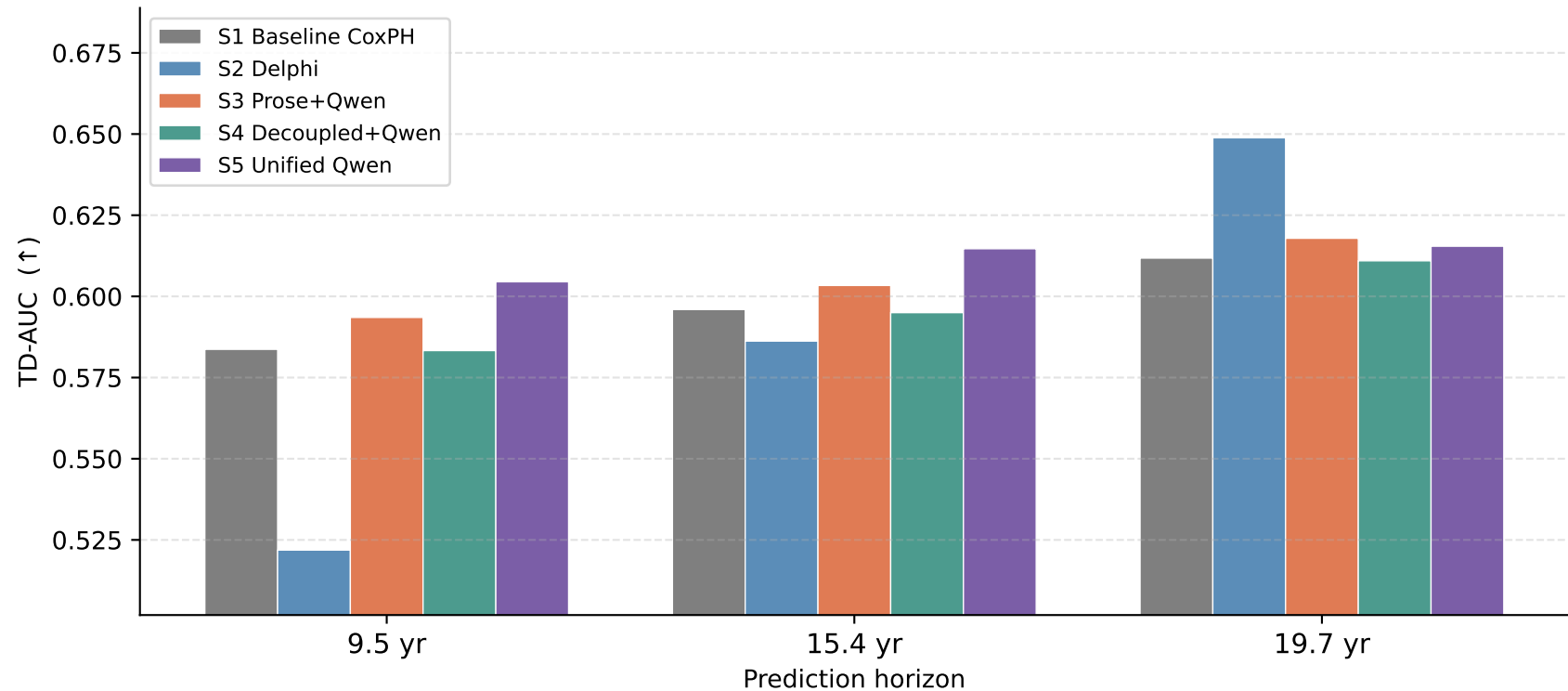
Time-Dependent AUC by Prediction Horizon (reference configurations, test n = 18,623)
