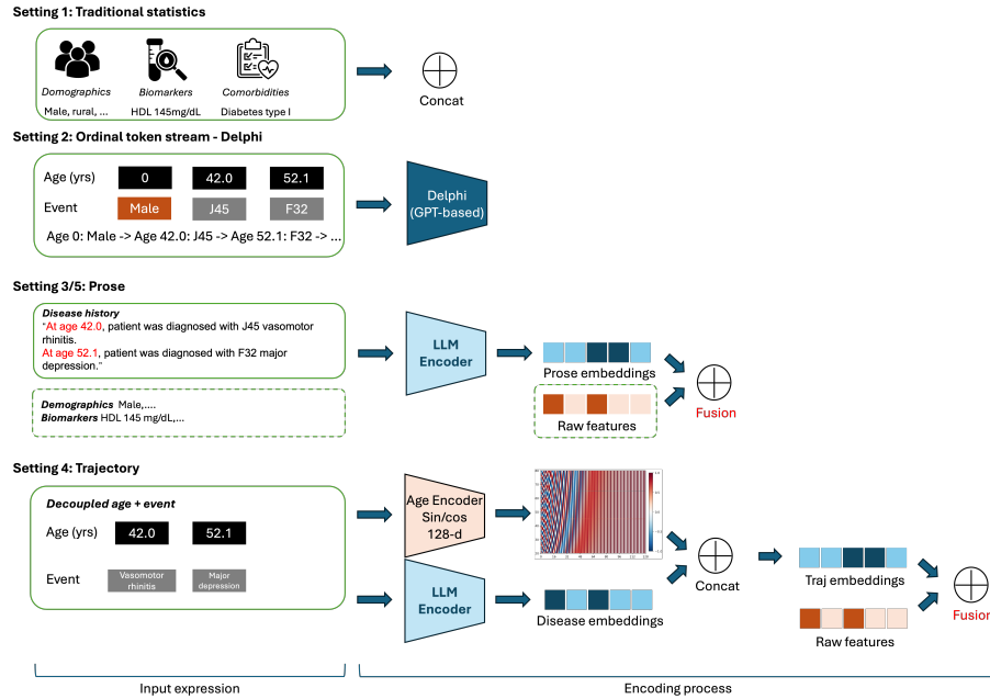
Fig. 2. Overview of the five experimental settings and their encoding pipelines. S1 (top): demographics, biomarkers, and comorbidities are concatenated into a fixed-dimension feature vector for CoxPH. S2 : age-tagged ICD tokens are fed to a GPT-based generative transformer (Delphi) in zero-shot mode. S3 : disease history is serialised as natural-language prose and encoded by a frozen LLM; the resulting embedding is fused with raw features. S4 : age values are mapped to a continuous sinusoidal encoding in parallel with ICD token embeddings; the two streams are concatenated per event, mean-pooled, and fused with raw features. S5 (bottom): all modalities are combined into a single paragraph and encoded by the LLM with no raw features concatenated.
