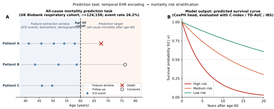
Fig. 1. Prediction task overview. (A) Three illustrative patient timelines from the UK Biobank respiratory cohort ( n=124,158 ). Blue dots mark ICD-10 diagnosis events before the age-60 feature-extraction cutoff; a red cross indicates death, an open circle indicates censoring. (B) Illustrative model output: a CoxPH survival curve S(t | x) stratified by predicted risk group. Evaluation metrics (C-index, TD-AUC, IBS) measure discrimination and calibration of these curves on the held-out test set.
