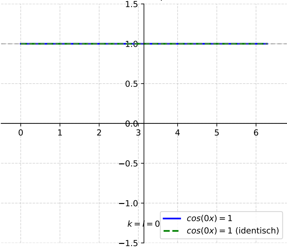
\cos(kx), \cos(lx) \mid l = k = 0
