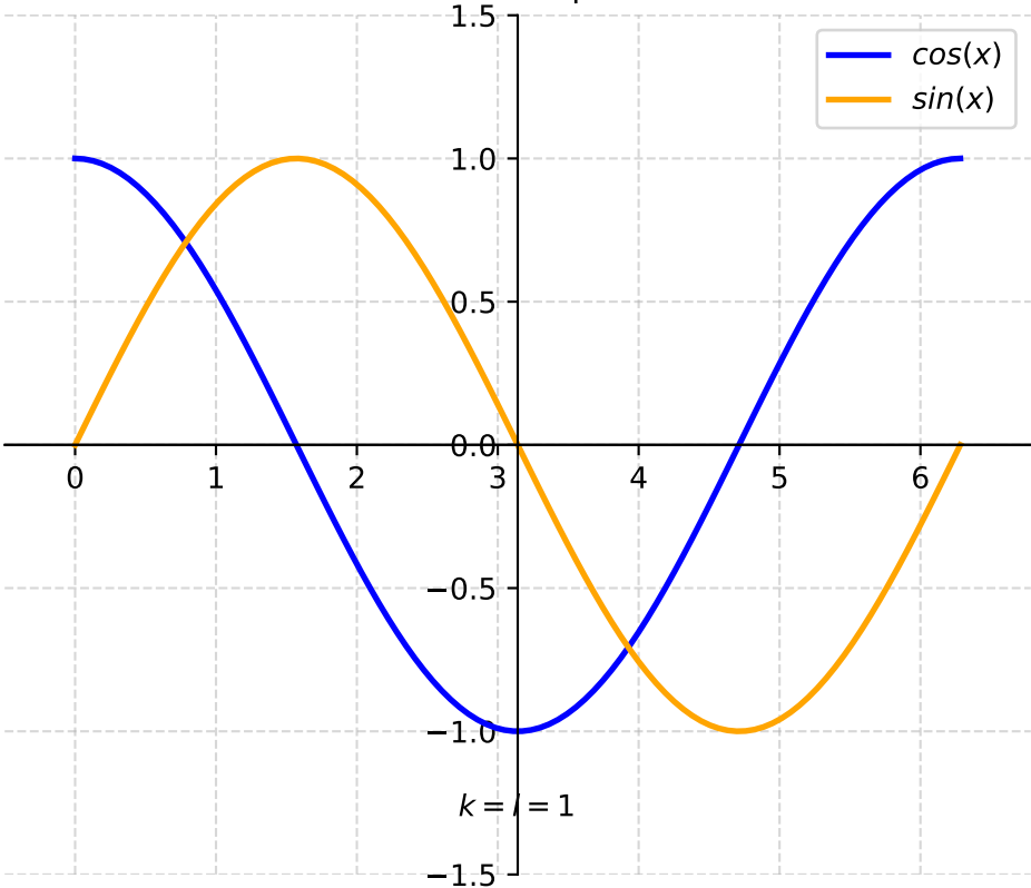
\cos(kx), \sin(lx) \mid l = k \neq 0
