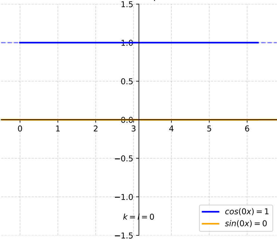
\cos(kx), \sin(lx) \mid l = k = 0
