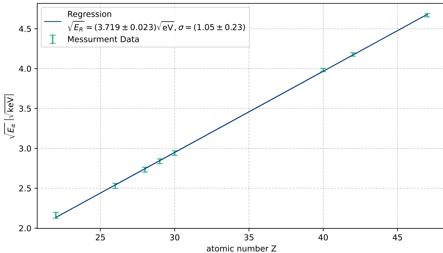
\sqrt{E_\alpha} as a function of Z
