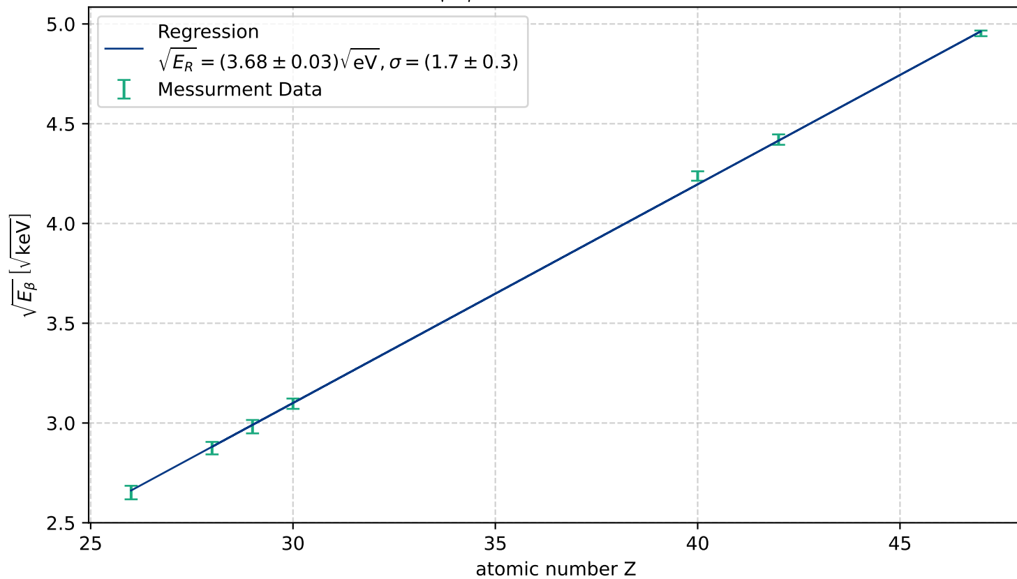
\sqrt{E_\beta} as a function of Z
