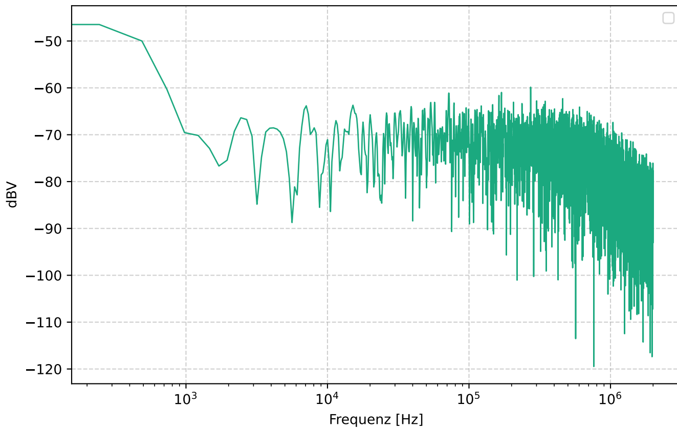
Frequenzgang (5k \Omega )
