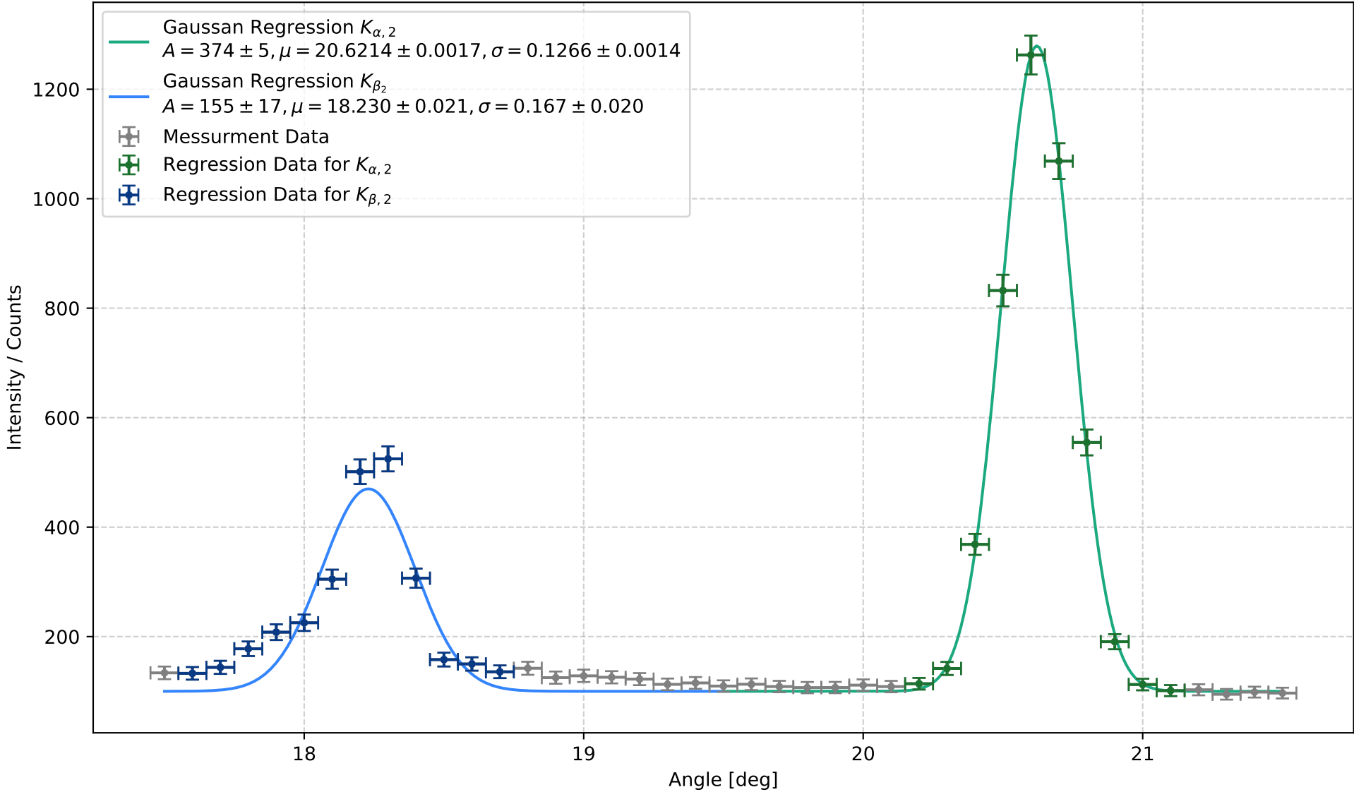
Second order K-Lines for Mo using the LiF Cristal
