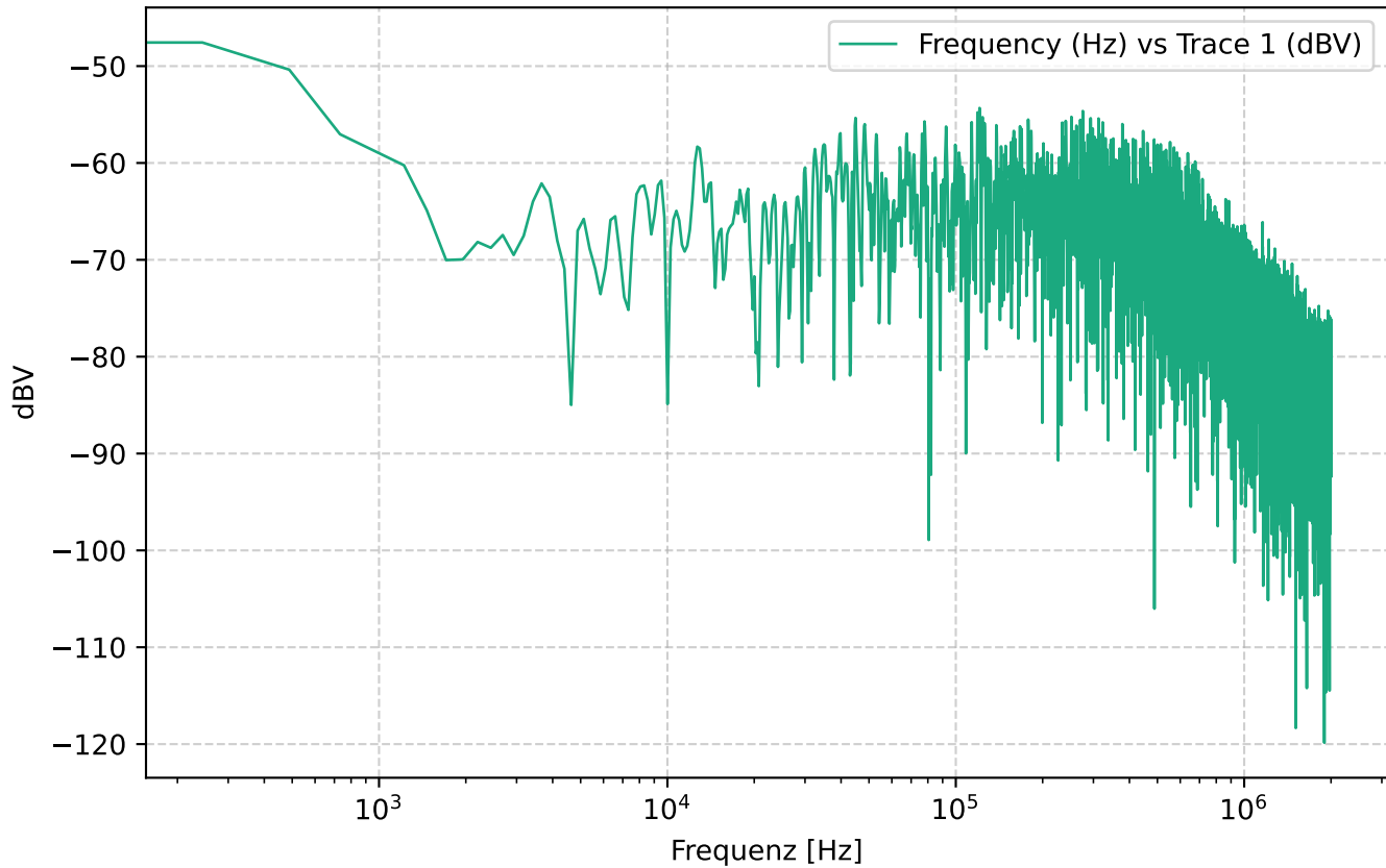
Frequenzgang
