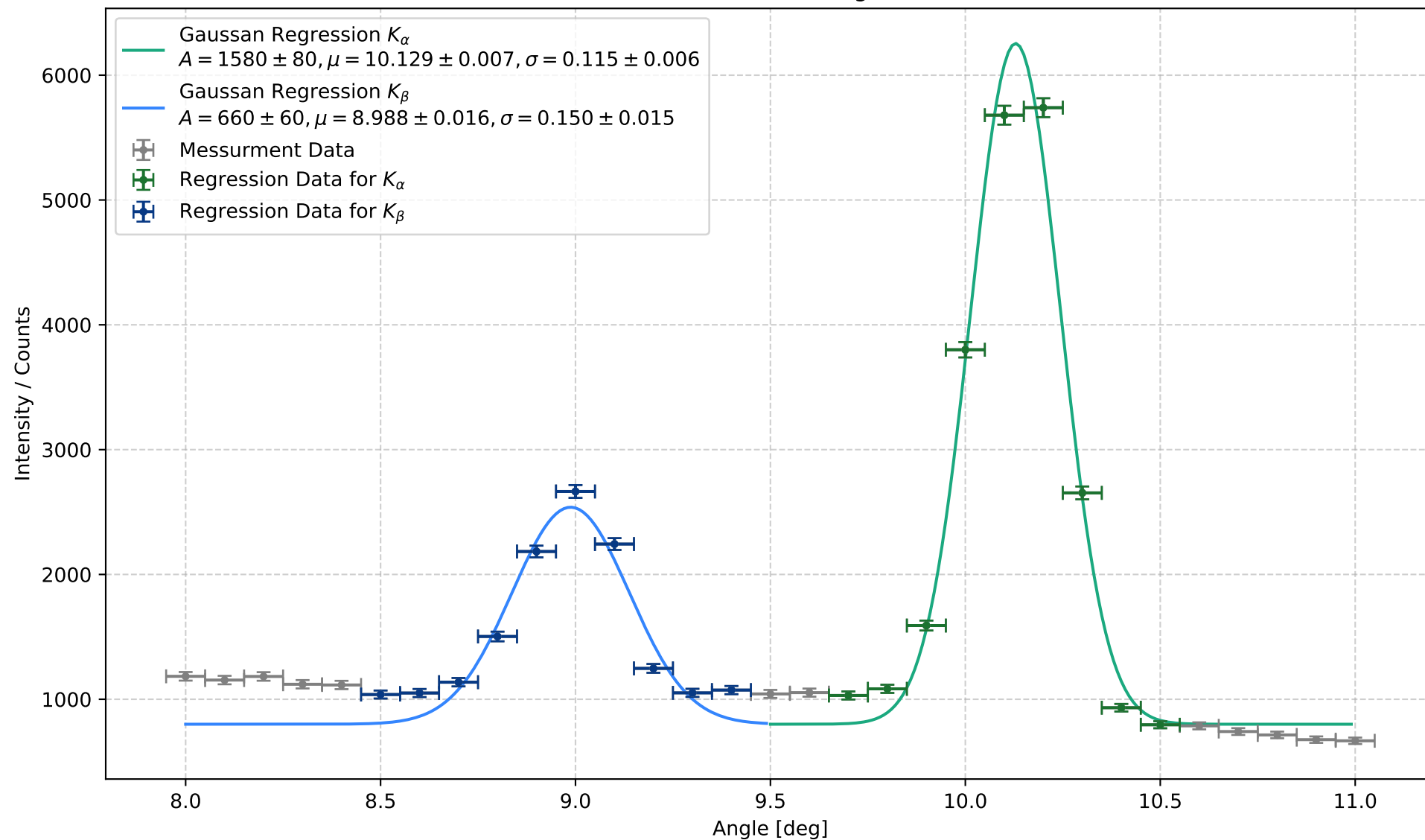
First order K-Lines for Mo using the LiF Cristal
