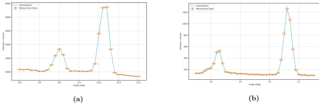
Figure 4.II: (a) High-resolution spectrum of the first-order and (b) second-order K-lines.
