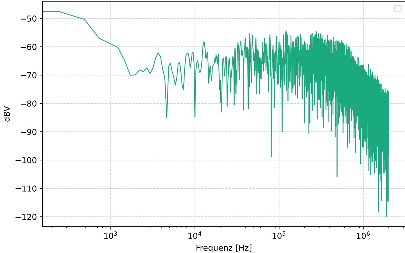
Frequenzgang
