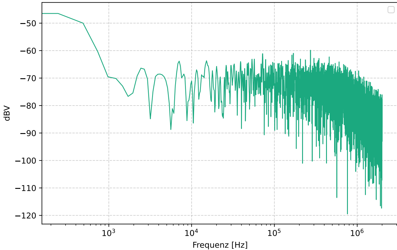
Frequenzgang (5k \Omega )
