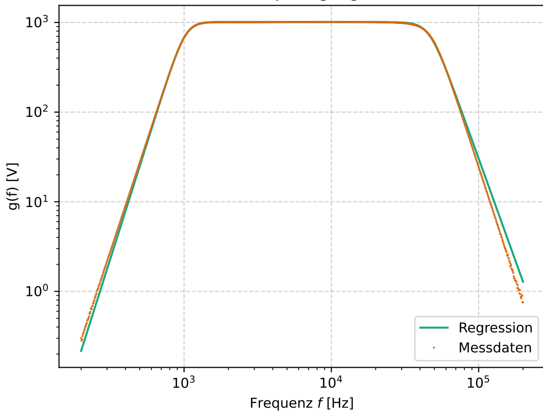
Frequenzgang
