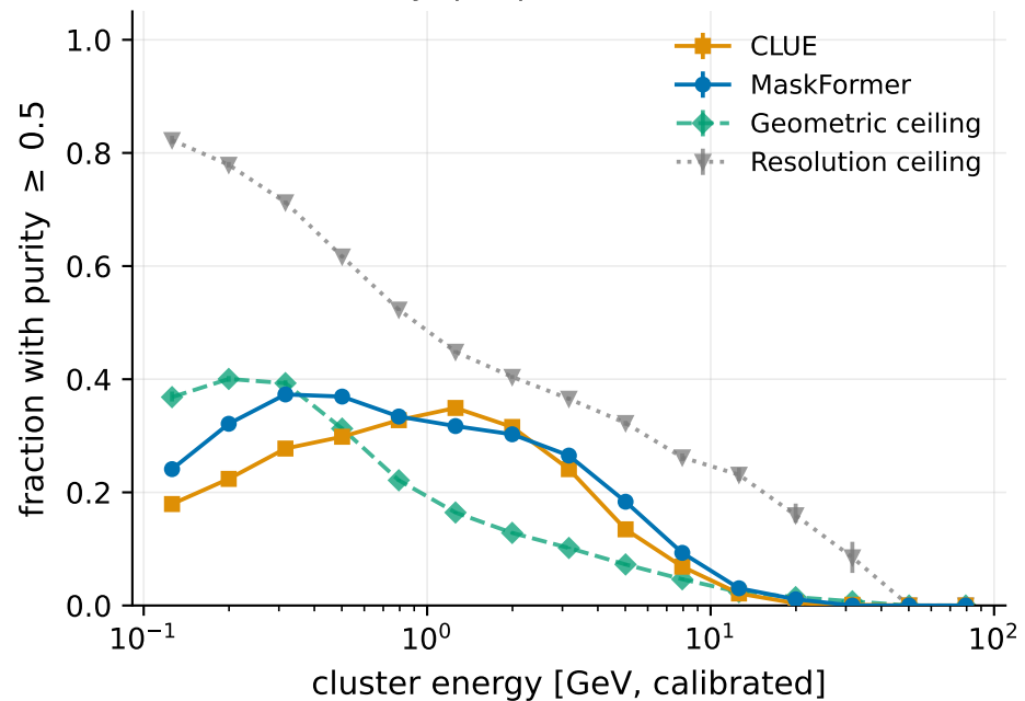
Purity (per predicted cluster)
