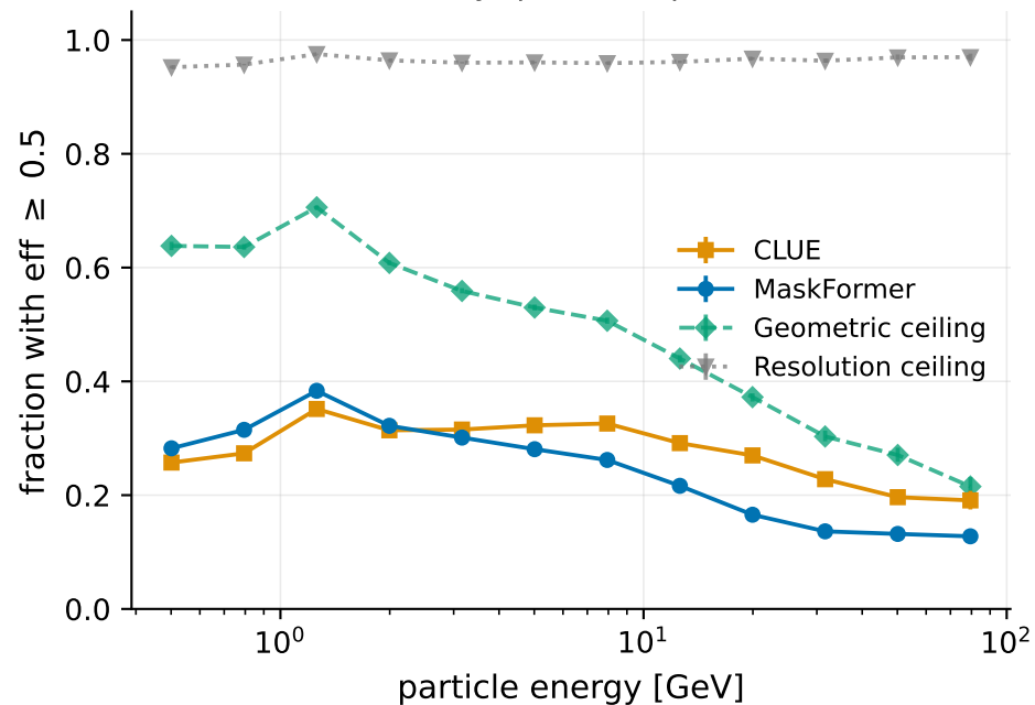
Efficiency (per truth particle)
