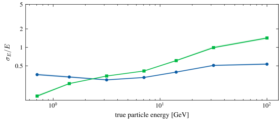
MaskFormer CLUE
