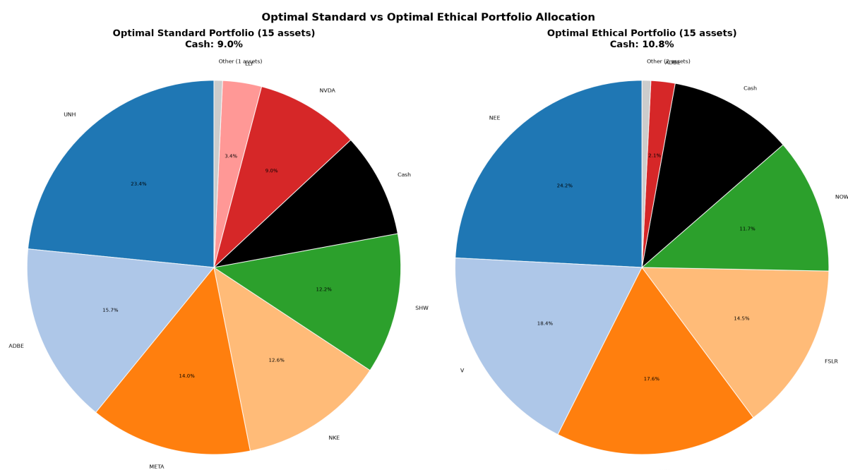
Figure 25: Optimal Standard (15 assets) vs Optimal Ethical (15 assets) Portfolio Allocation
