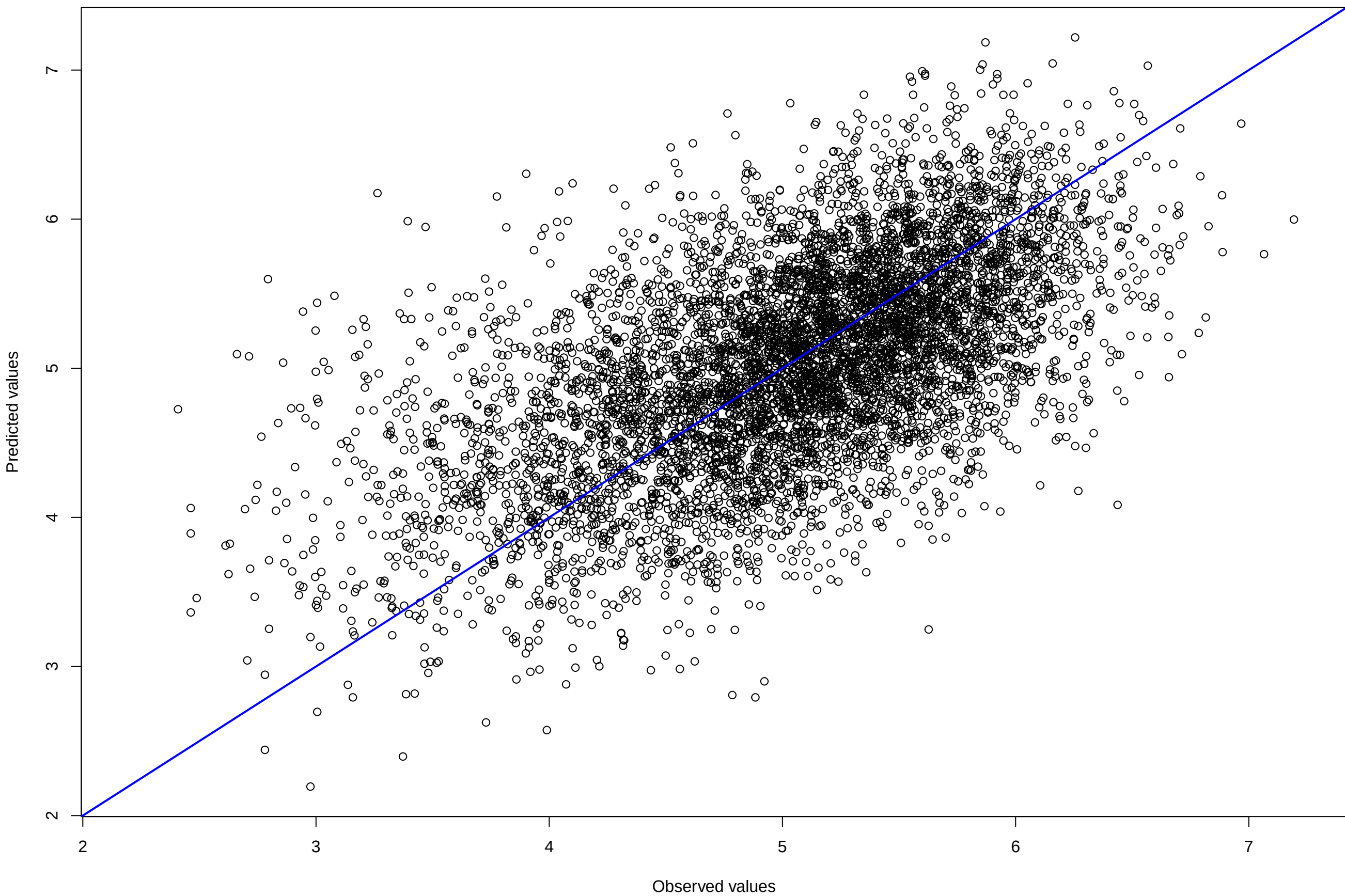
Observed vs predicted (Posterior Mean with Simulated Noise)
